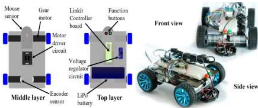
Figure 1. Physical view of the robot (a) fully assembled mobile robot diagram (b) Fully assembled mobile robot images
