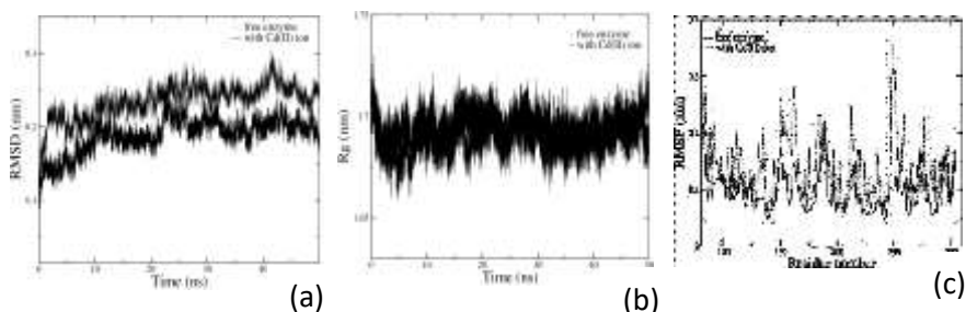
Figure 4. The structural behavior of the enzyme with and without the Cd (II) ion. (a) RMSD (b) Rg (c) RMSF
