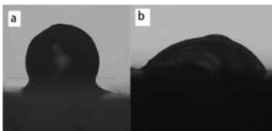
Figure 4. Images of solder droplets taken (a) without the ZnCl_2/HCl treatment (b) with the ZnCl_2/HCl treatment
