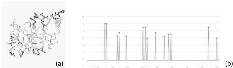
Figure 2. MIB server results for the enzyme hUNG with the Cd (II) ion. (a) Metal ion binding residues are shown as sticks in the protein image. (b) Predicted scores as the binding potential for the residues of the enzyme hUNG.
