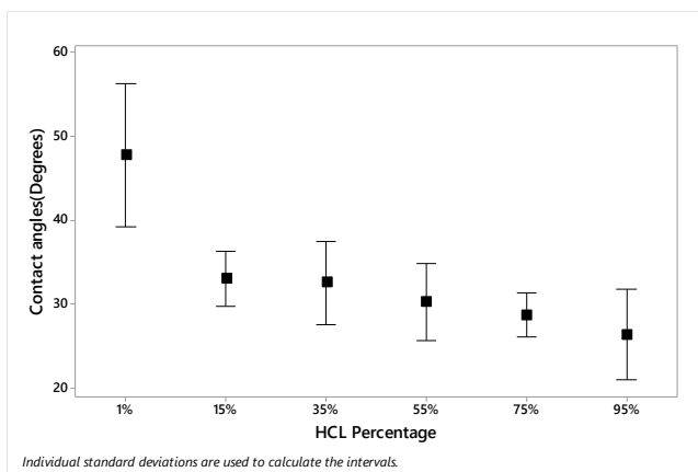
Figure 5. Resultant contact angle values of solder droplets after the treatment of \text{ZnCl}_2/\text{HCl} by changing the HCl content.
