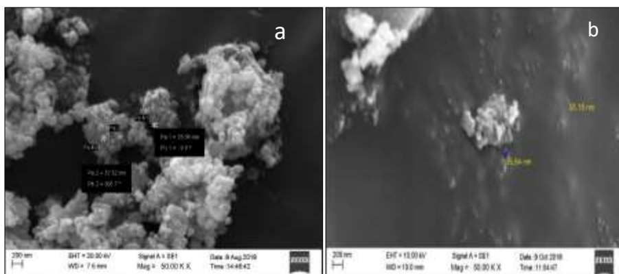
Figure 1. TiO 2 particle size (a) without triton X-100 (b) with triton X-100
