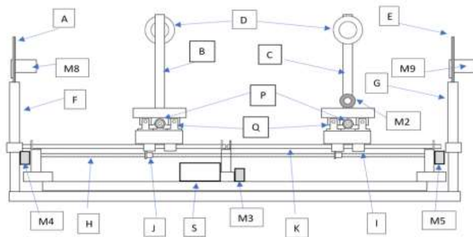
Figure 2. Side View of the robot
